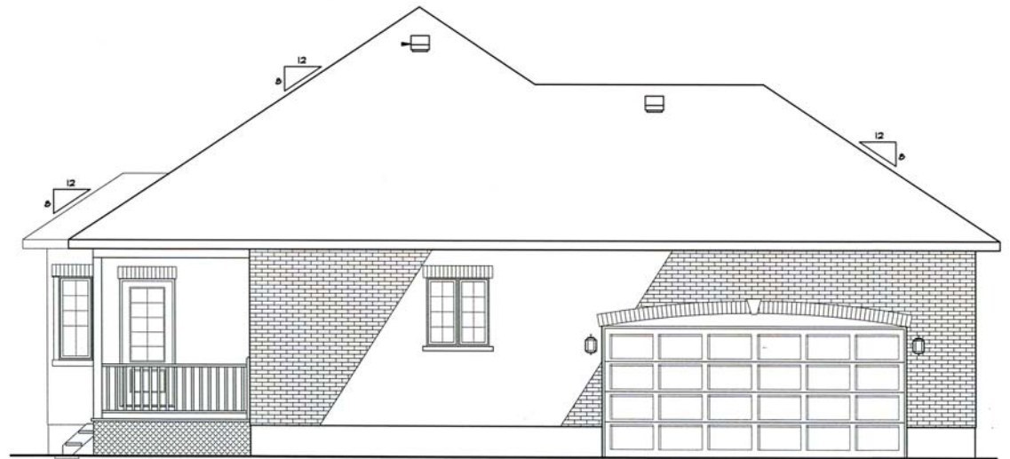
South Elevation
